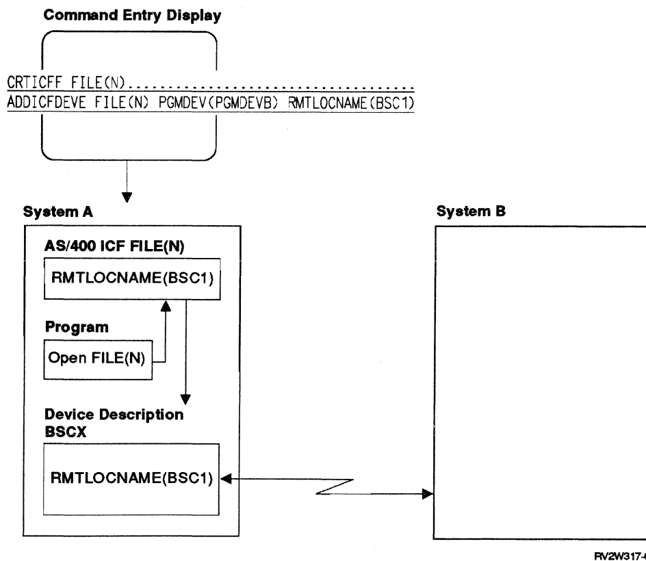
Figure 2-5. Non-APPC Communications
